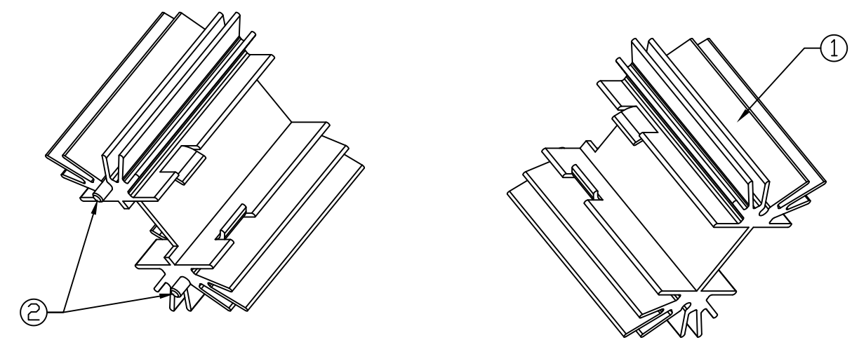
ISOMETRIC VIEW SCALE 1:1
