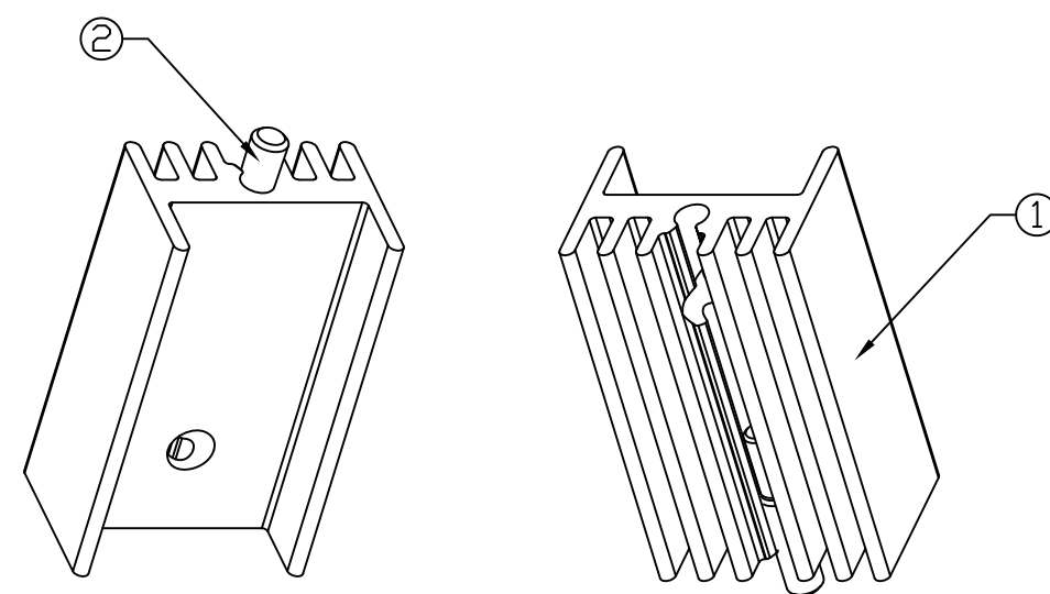
ISOMETRIC VIEW SCALE 2:1
