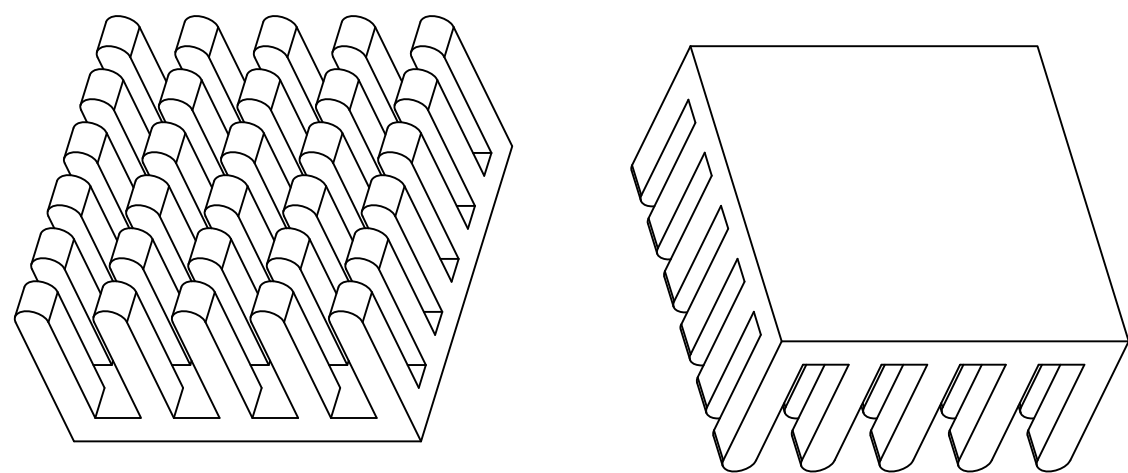
ISOMETRIC VIEW SCALE 2:1
