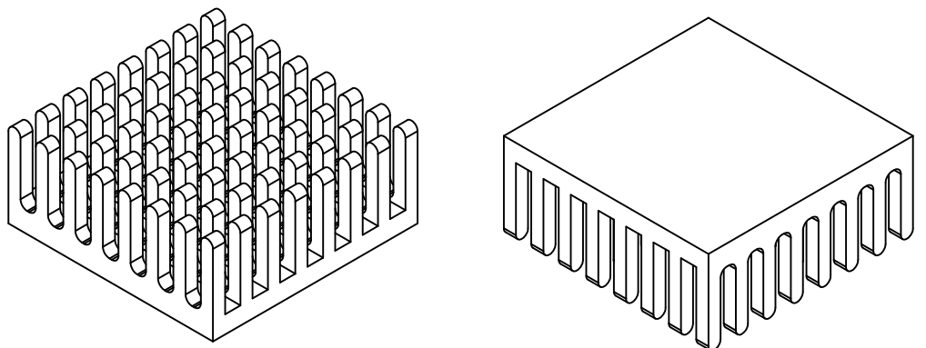
ISOMETRIC VIEW SCALE 2:1
